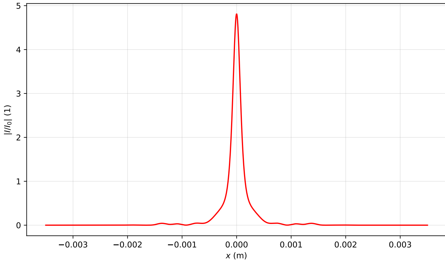
Intensity profile I(x, y = 0, z = 1.672)/I_0 , P_{in}=4.5P_{cr} , artificial time
